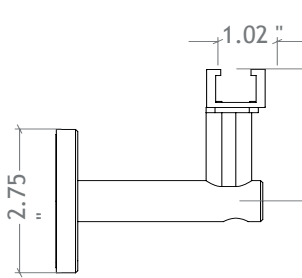
Wall-Mount
