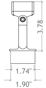
Post Mount
